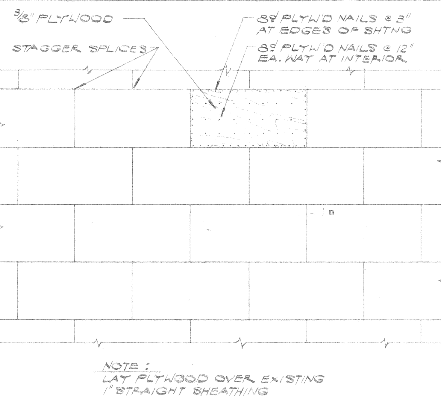
PLYWOOD SHEATING DETAIL
