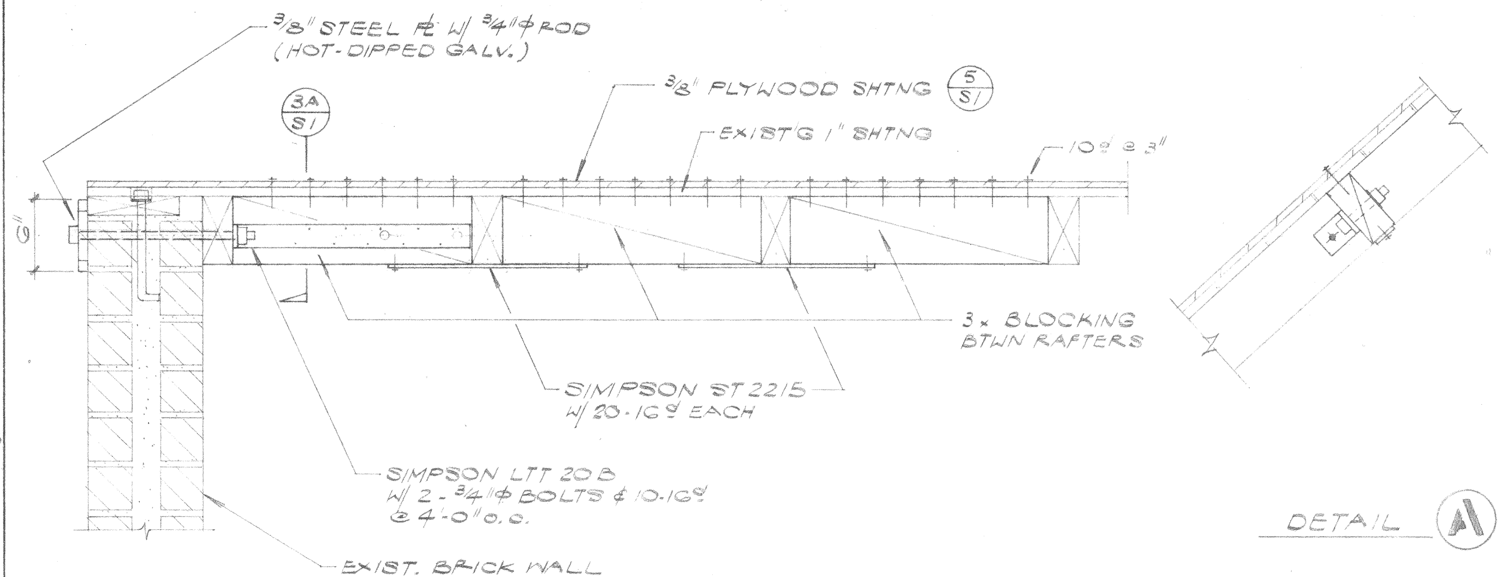
ROOF SECTION AT RAKE
