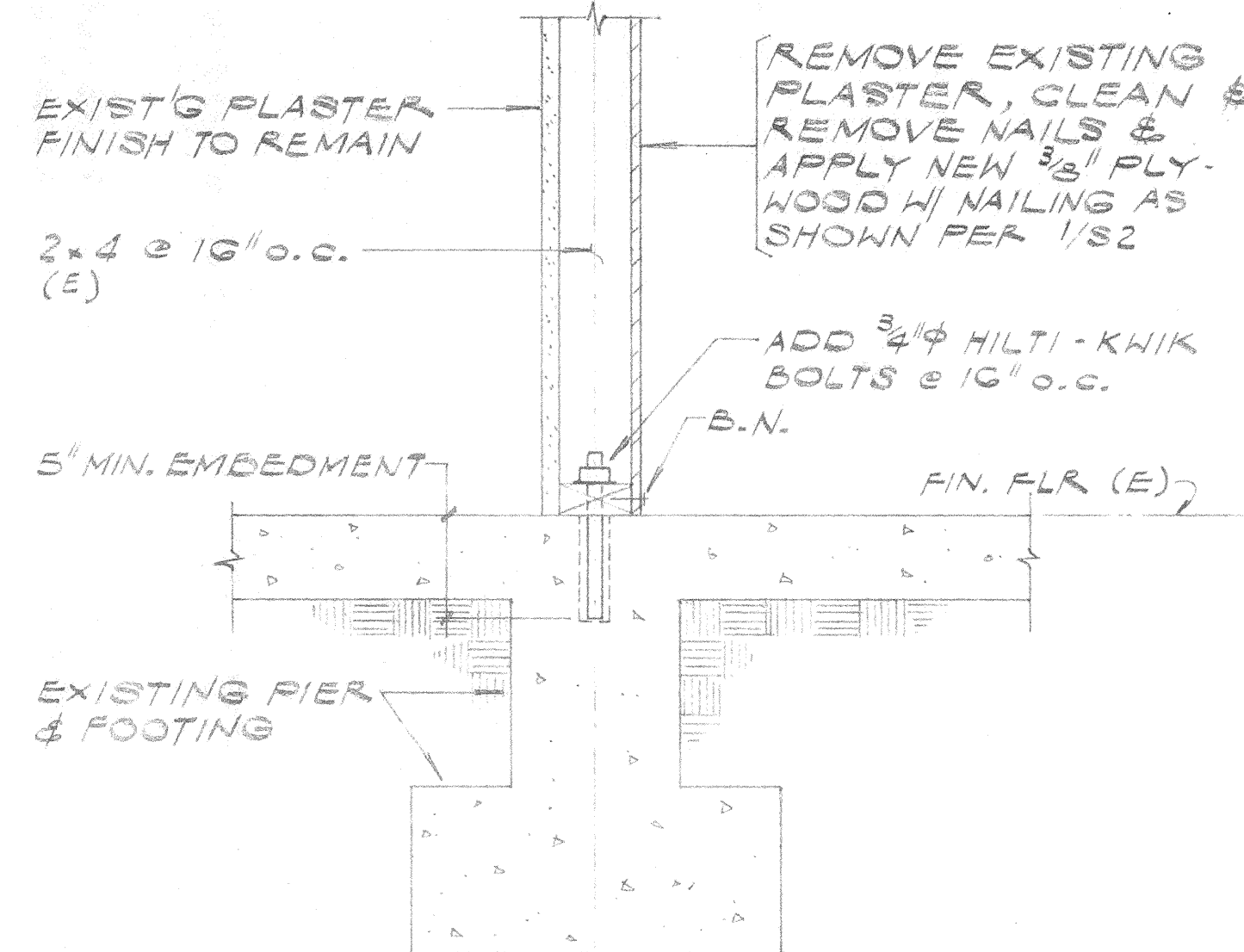
SECTION AT SHEAR WALL
