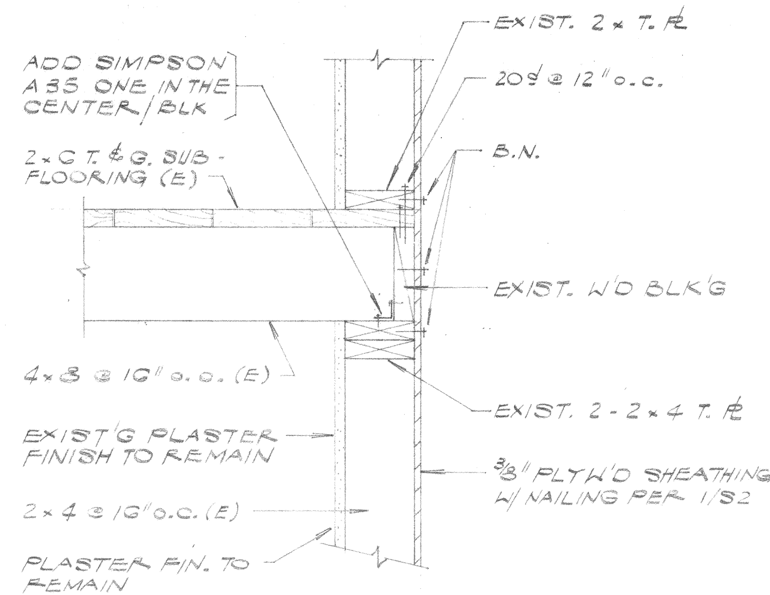
SECTION AT 2nd FLOOR
