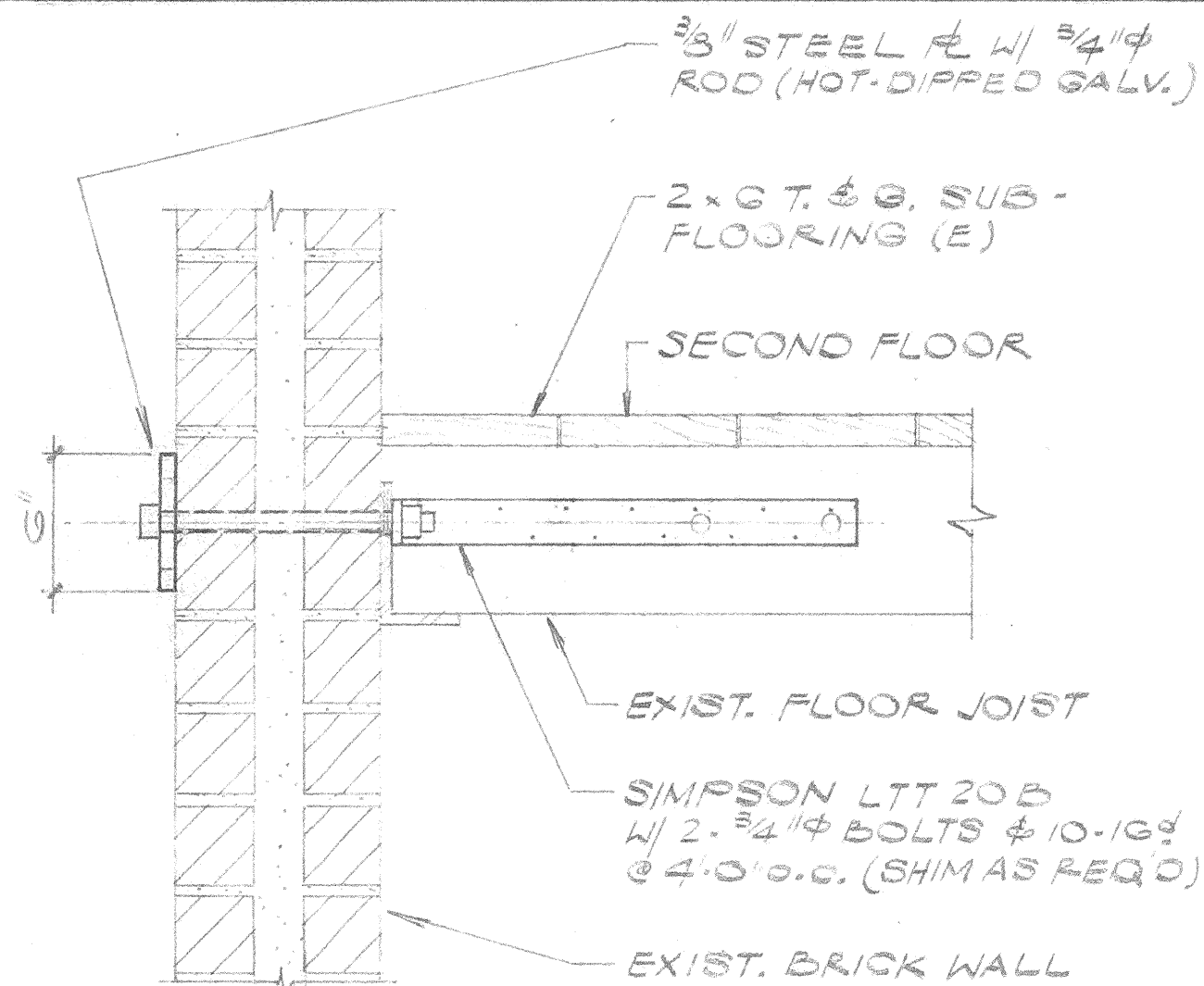
SECTION AT SHEAR WALL
